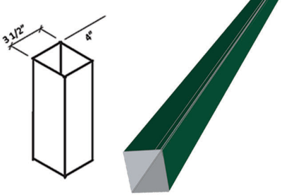
DOWNPOUT 16 1/2" W
